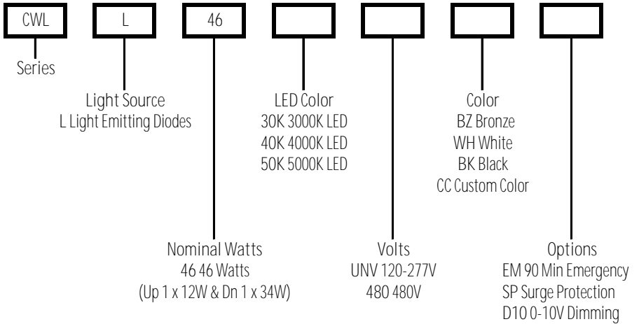
CWL Up/Down LED Series
