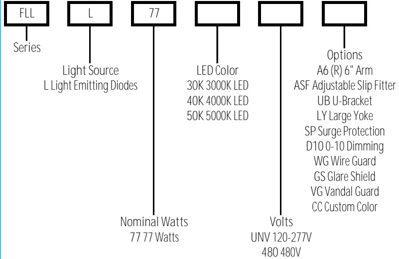
FLL LED Series
