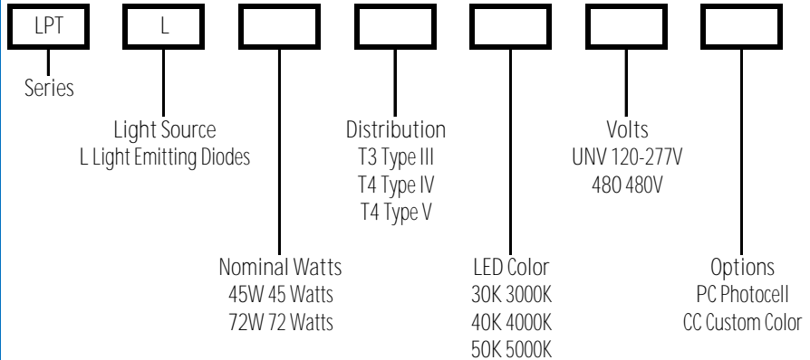
LPT LED Series
