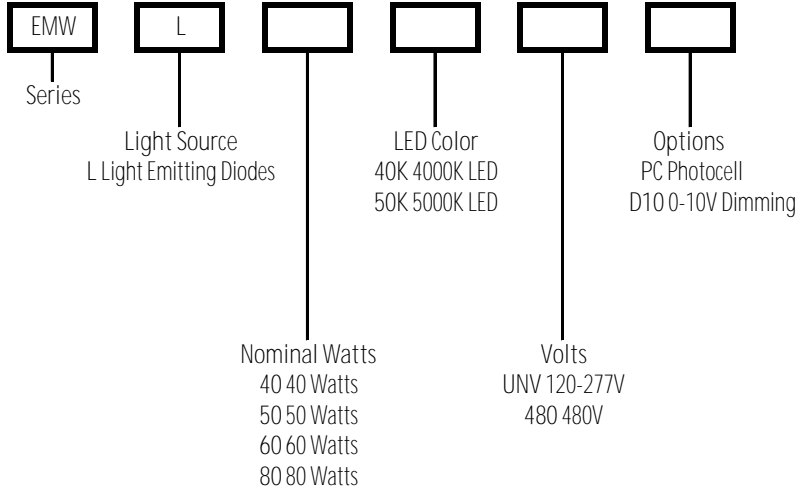
EMW LED Series
