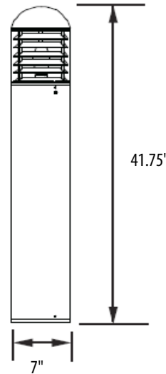
DBB Direct Bury Base
